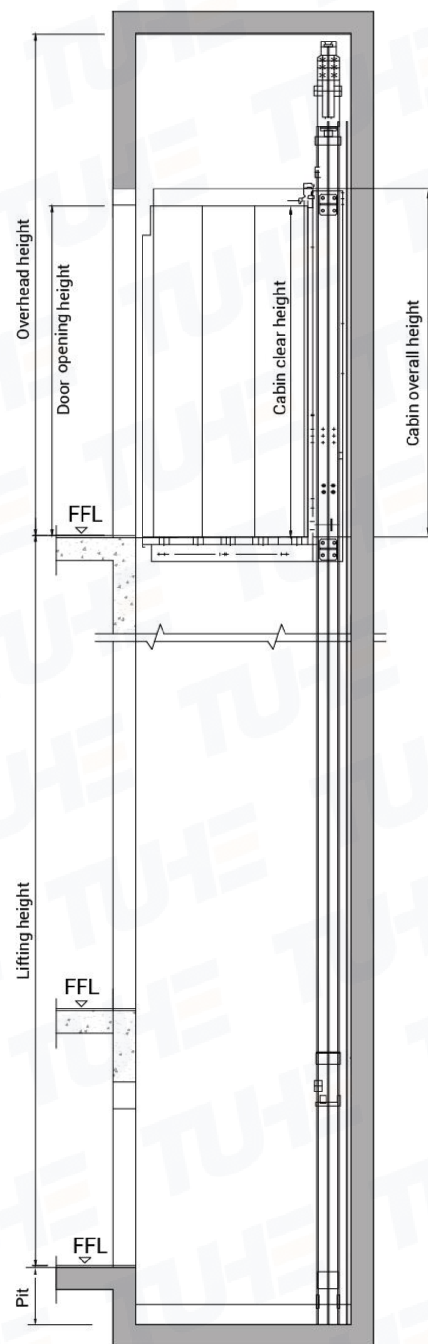
SIDE VIEW
