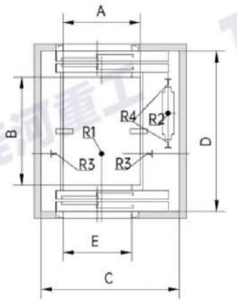
井道平面图(180度贯通门) Shaft plain drawing(Through door opening)
